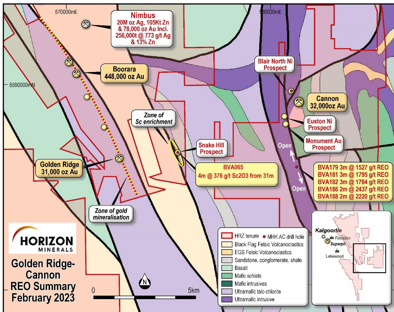
Figure 2: Golden Ridge – Cannon drilling REE highlights
