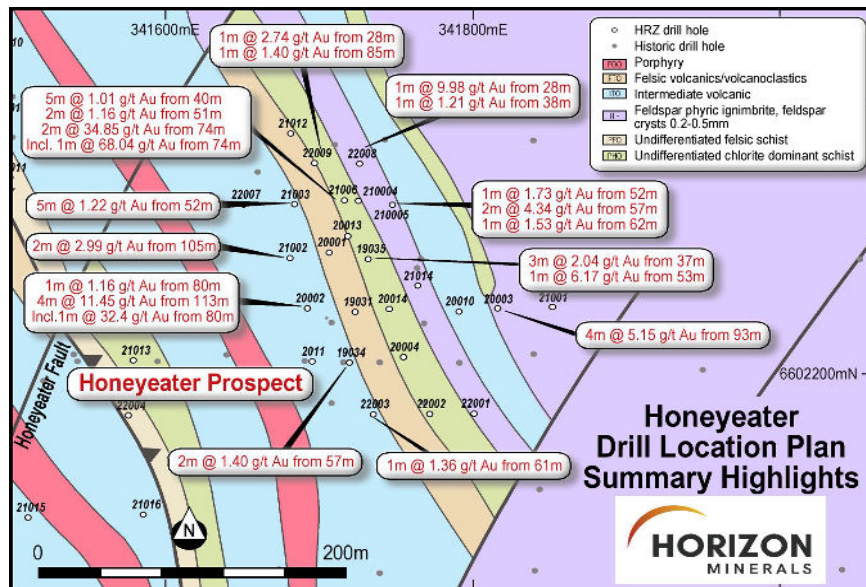
Figure 10: Honeyeater prospect geology and drilling highlights
