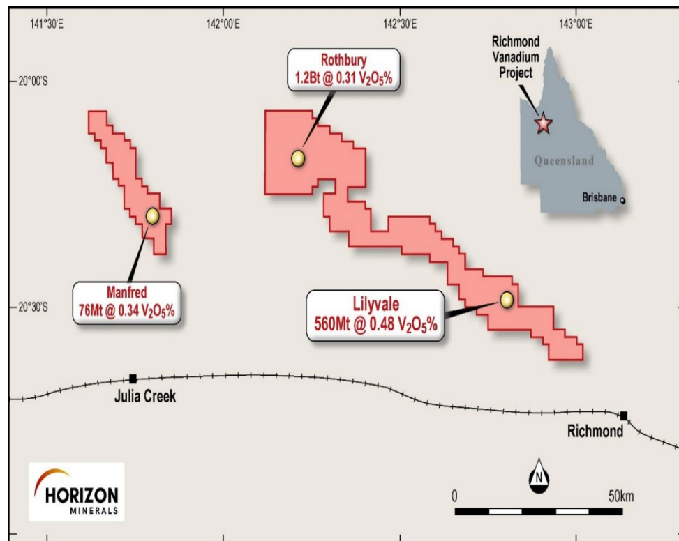
Figure 21: Lilyvale Vanadium project location and Richmond Lease areas
