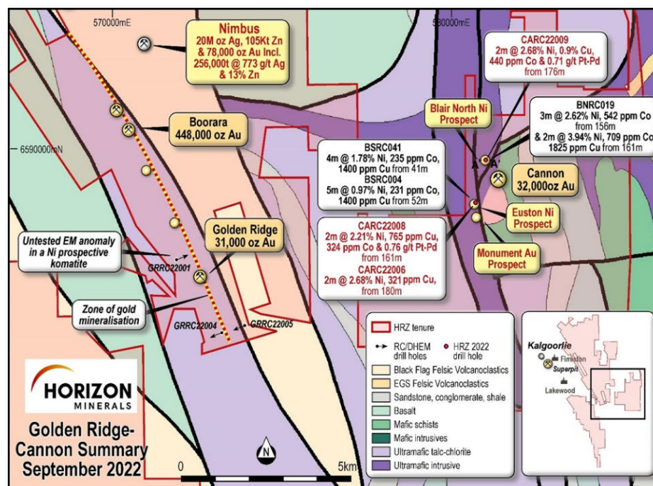
Figure 8: Blair North and Euston drilling results and local geology
