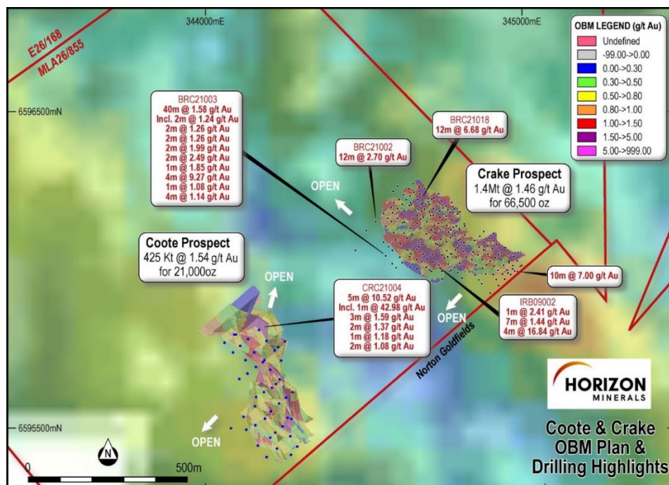
Figure 9: Magnetic Image with drilling highlights at Coote and Crake
