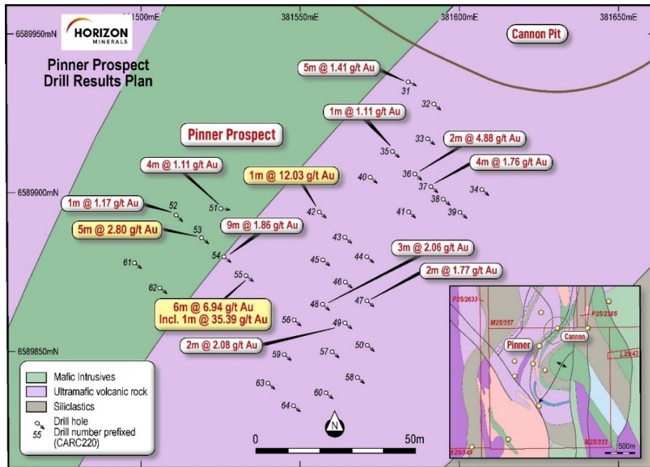
Figure 7: Pinner gold prospect drilling highlights
