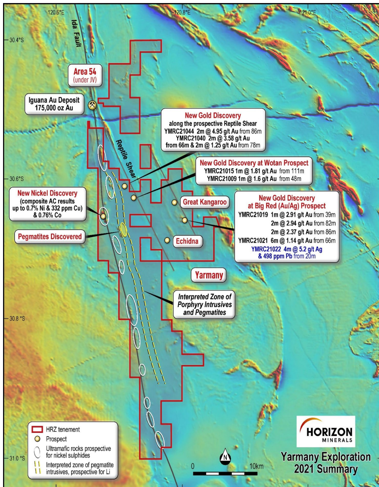
Figure 15: Regional Magnetic Image with the 2021 Yarmany Exploration Highlights
