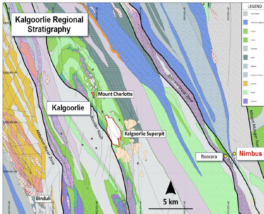
Figure 18: Nimbus project location and regional geology
