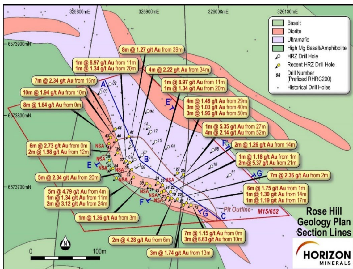
Figure 12: Rose Hill drill hole 2020 collar plan and cross section locations
