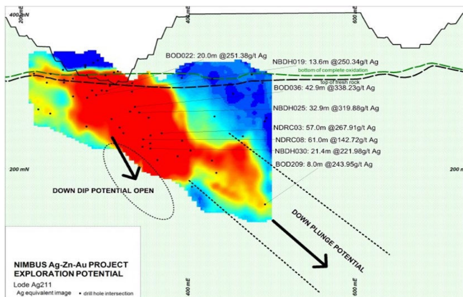
Figure 19: Long section through Ag Lode 211 showing down dip/plunge extension
