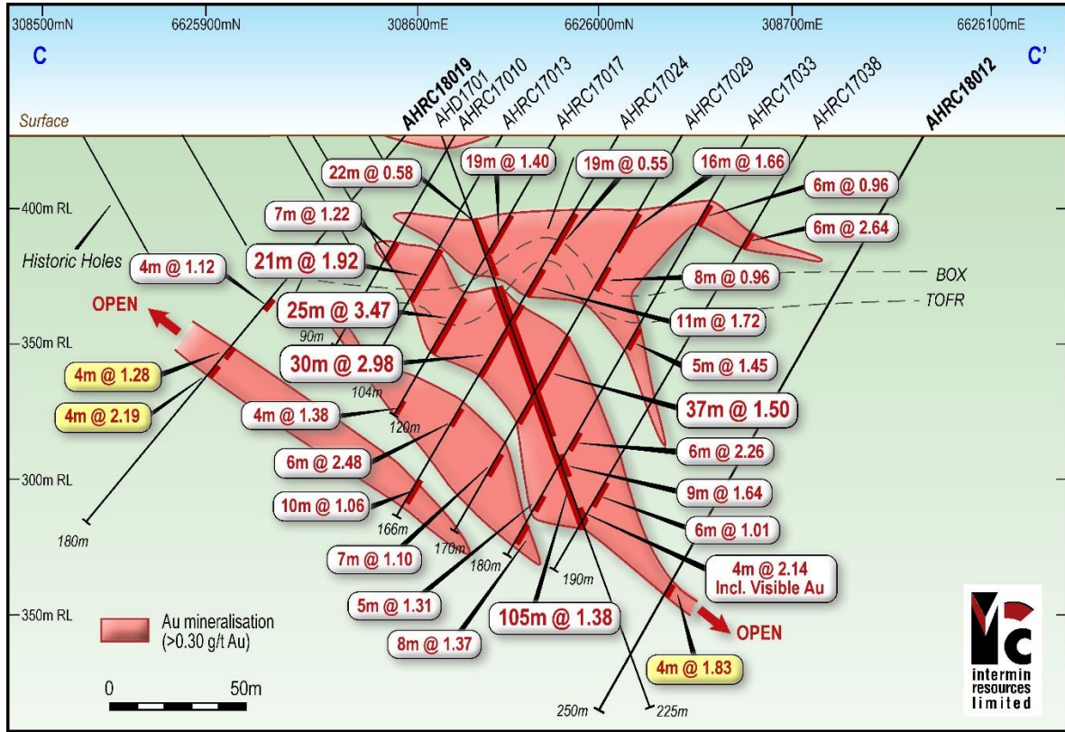
Figure 10: Anthill prospect cross section C-C' (see Figure 7 for reference) 1
