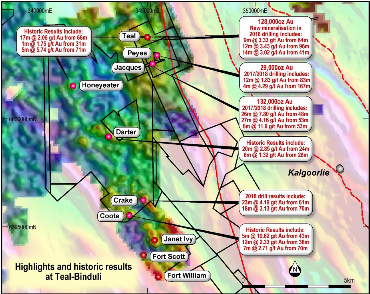
Figure 6: Teal and Binduli project areas overlying TMI and regional gold (ppb) geochemistry 1,2
